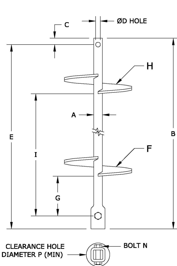
FIGURE 1A—SS5 & SS175 LEAD SECTIONS
