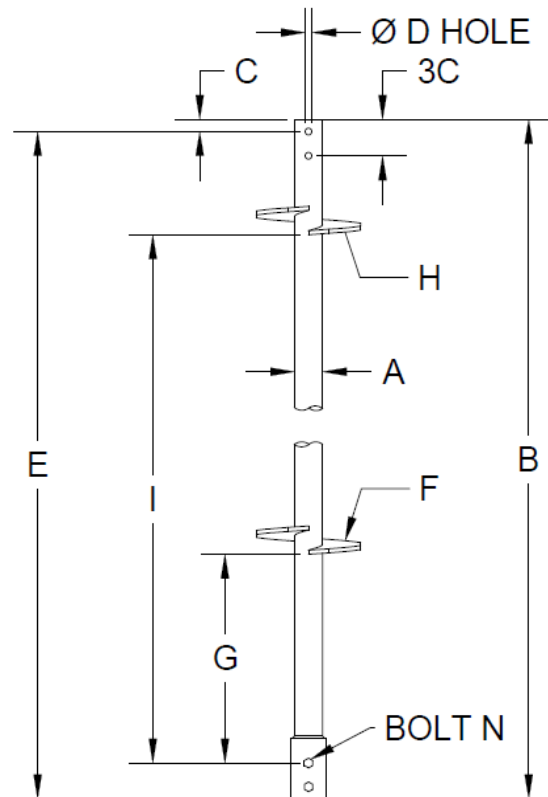
FIGURE 2B—RS2875.203, RS2875.276, RS3500 & RS4500 EXTENSION SECTIONS (RS4500 not shown)
